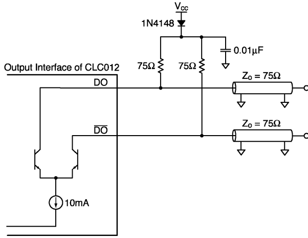
FIGURE 6. Differential Source Terminated Output Interface
