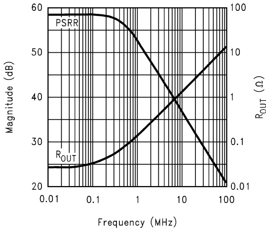
PSRR & R_{OUT}
