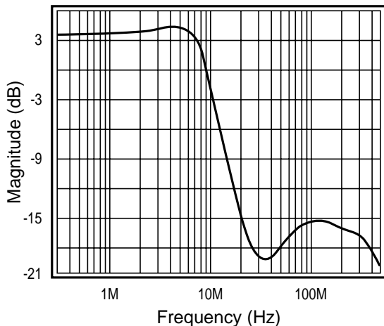
FIGURE 14. Lowpass Response
