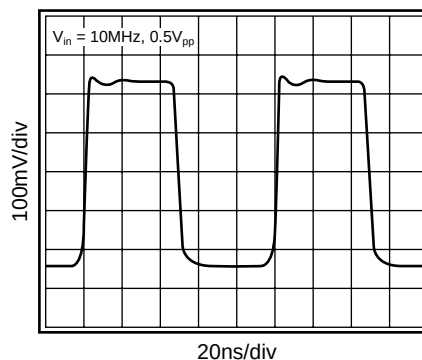
Figure 14: Single Supply Cable Driver
