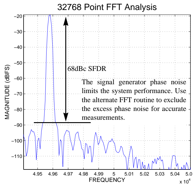
Figure 17 IF Input = 150MHz at 0dBm, Close-up
