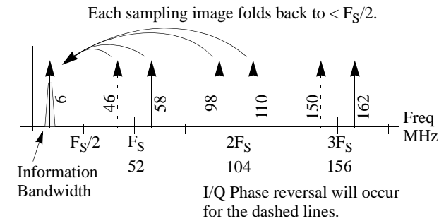
Figure 2 Sub-Sampling
