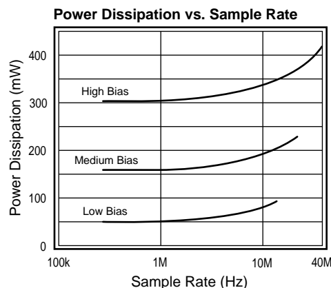
Figure 5: Power Dissipation vs. Sample Rate
