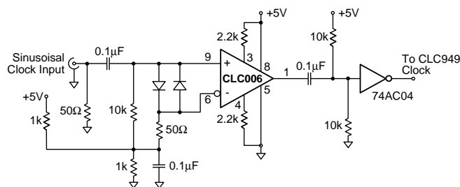
Figure 2: Clock Generation
