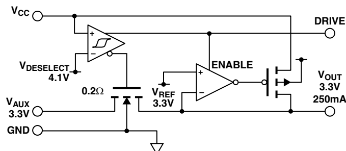
Simplified Electrical Schematic
