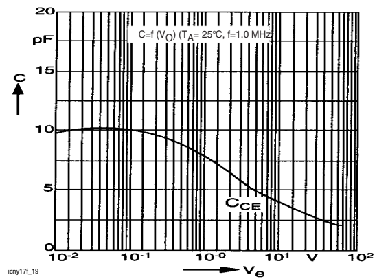
Figure 19. Transistor Capacitance
