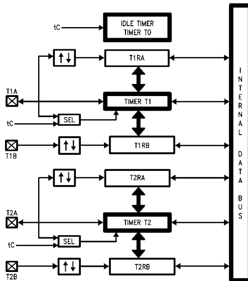
FIGURE 7. Timers
