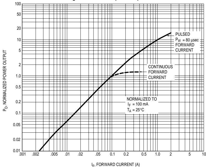
Figure 1. Power Output vs. Input Current
