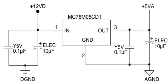
Figure 26. +5V Analog Voltage Regulator
