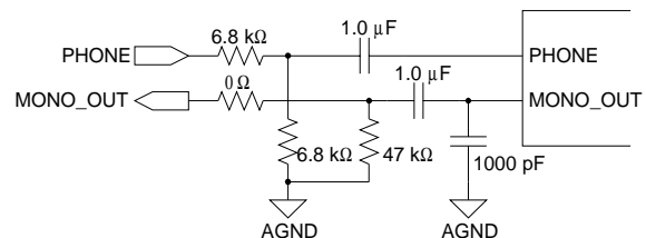
Figure 23. Modem Connection
