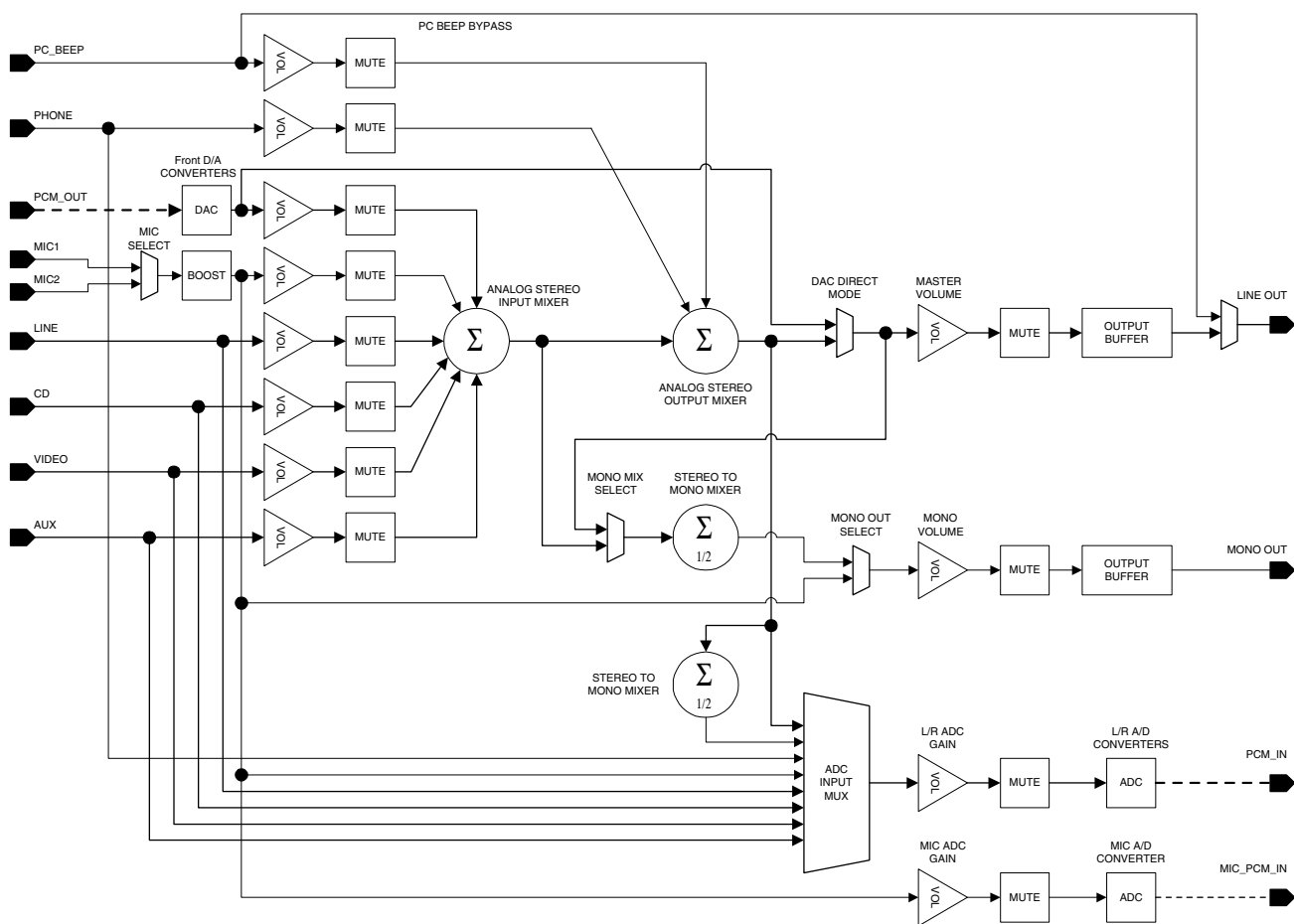
Figure 8. CS4205 Mixer Diagram
