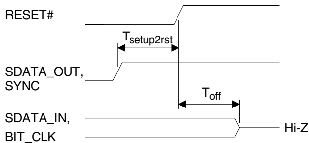
Figure 6. Test Mode
