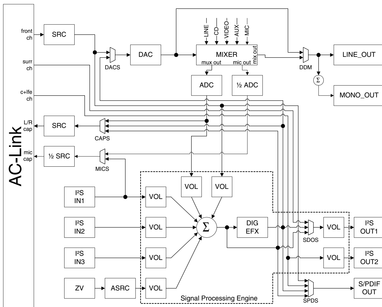
Figure 9. Digital Signal Path Overview
