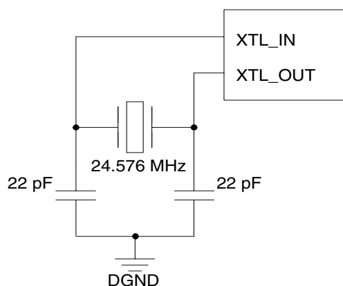
Figure 24. External Crystal
