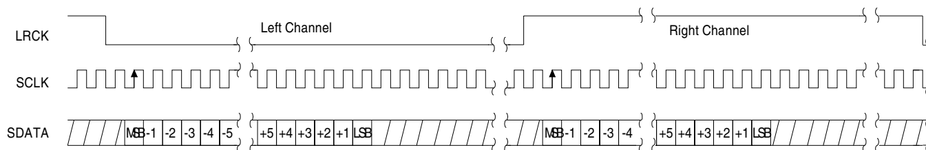
Figure 17. Serial Data Format 0 (I²S)
