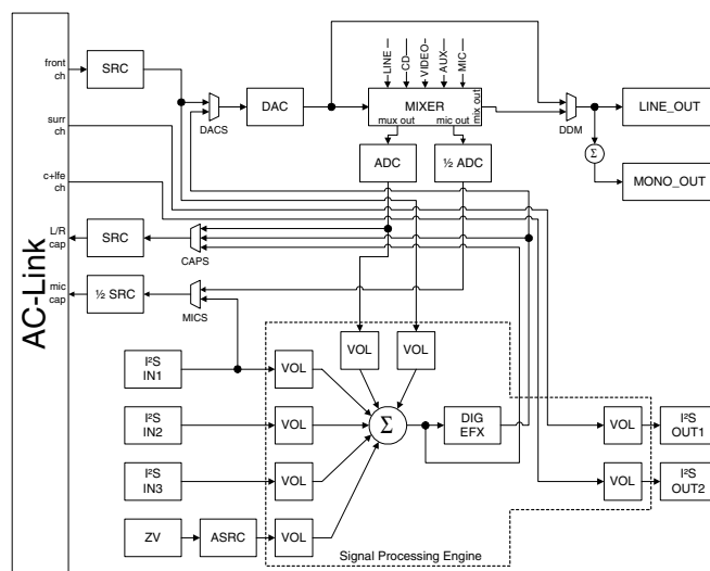
Figure 13. Multi-Channel Mode
