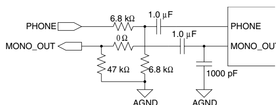
Figure 30. Modem Connection
