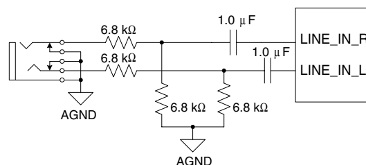
Figure 25. Line Input (Replicate for Video and AUX)
