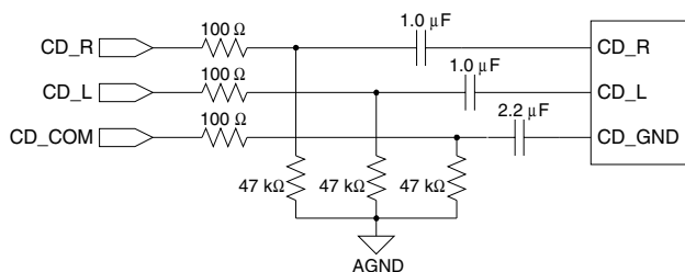
Figure 27. Differential 1 V RMS CD Input
