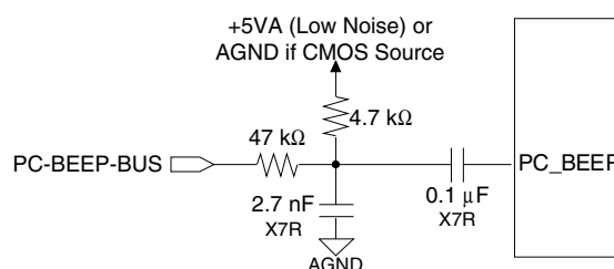
Figure 29. PC_BEEP Input
