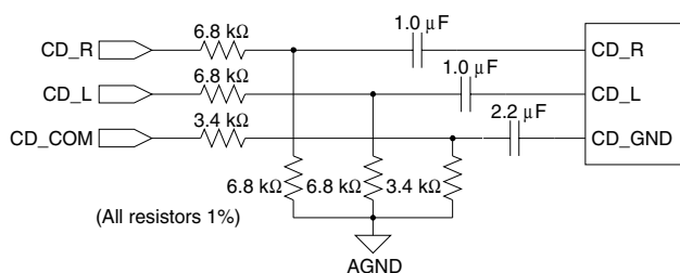
Figure 26. Differential 2 V RMS CD Input
