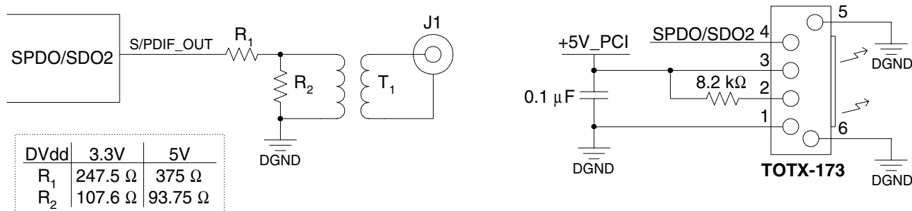
Figure 22. S/PDIF Output
