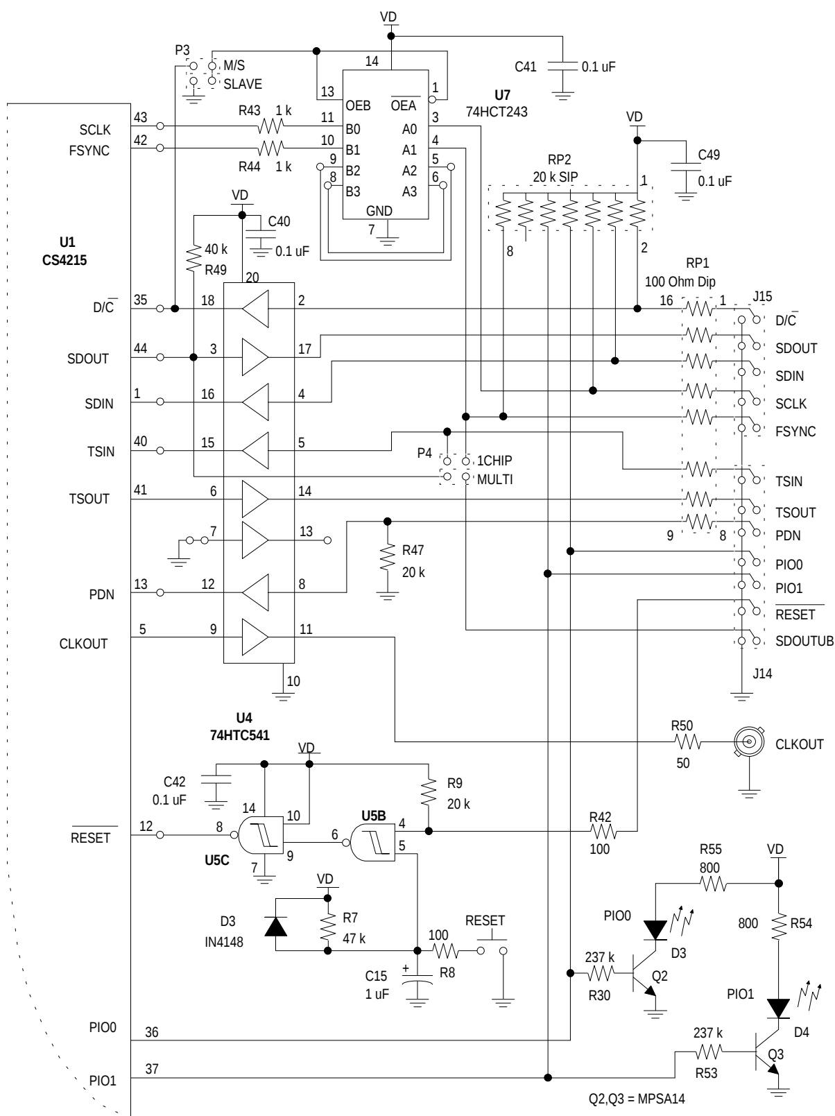
Figure 4. Digital Interface
