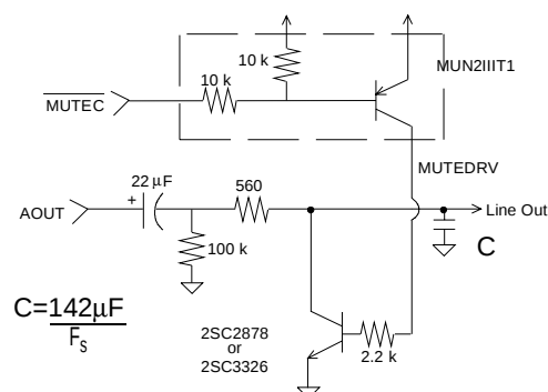
Figure 7. Passive Output Filter with Mute
