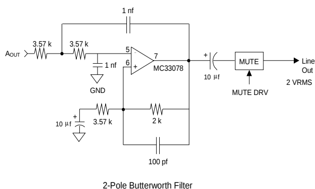
Figure 8. Butterworth Output Filter with Mute
