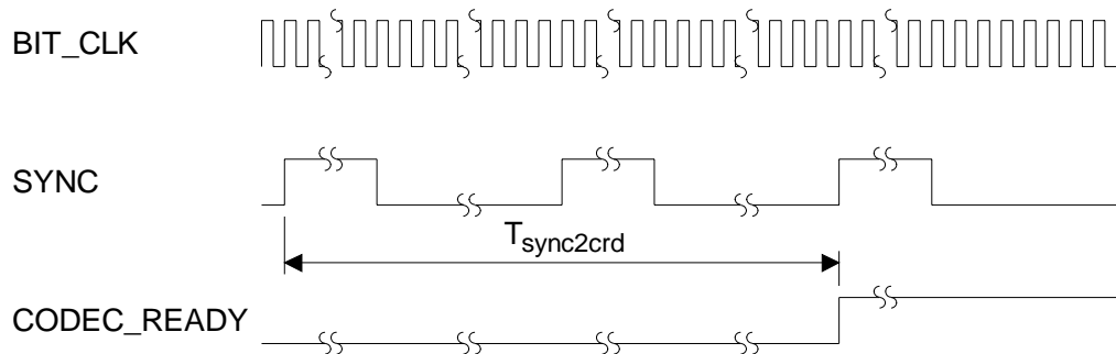
Figure 2. Codec Ready from Startup or Fault Condition
