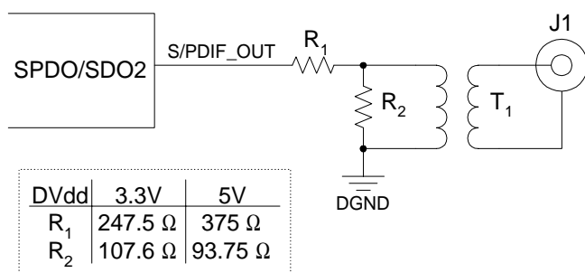
Figure 20. S/PDIF Output
