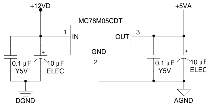
Figure 19. Voltage Regulator
