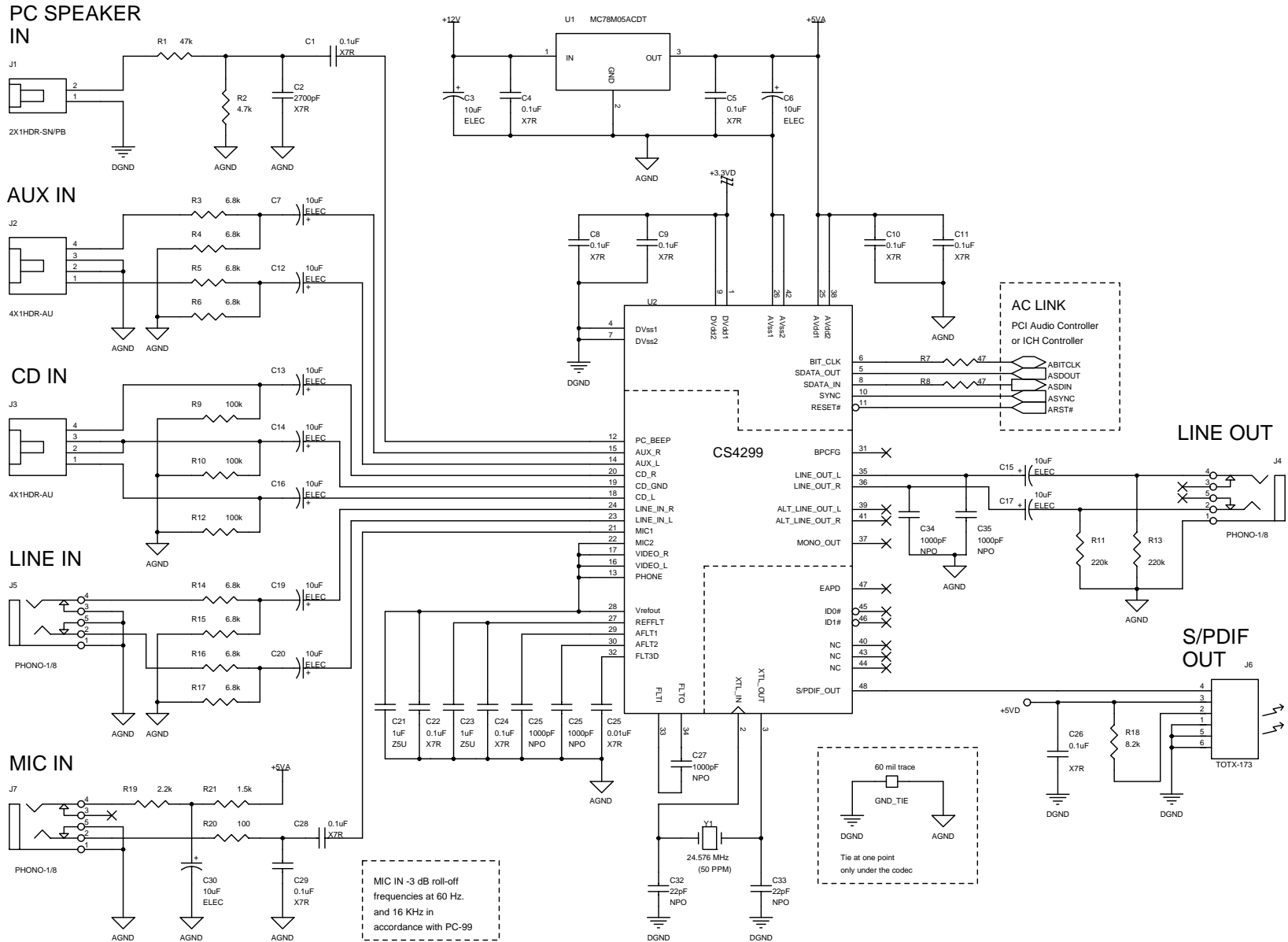
Figure 23. CS4299 Reference Design
