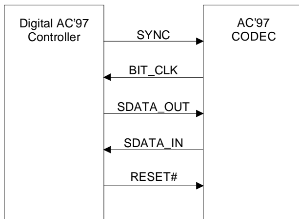
Figure 7. AC-link Connections
