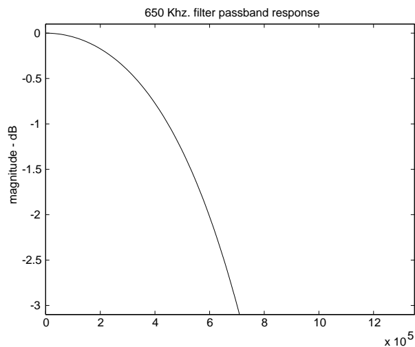
Figure 17. 650 kHz Chrominance low-pass filter transfer characteristic (passband)
