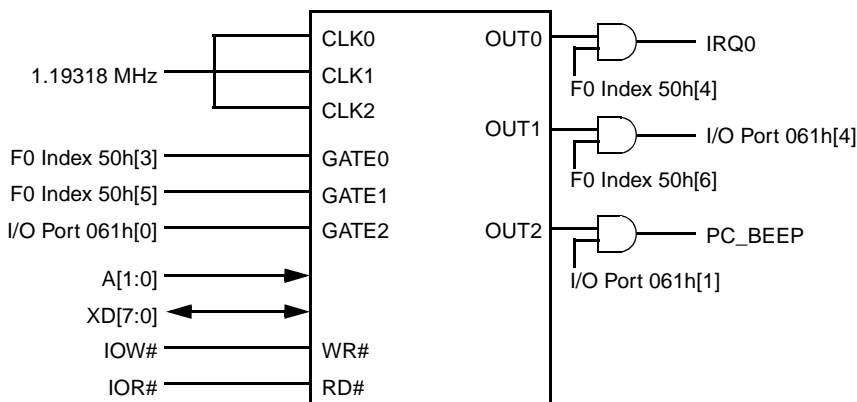
Figure 3-14. PIT Timer
