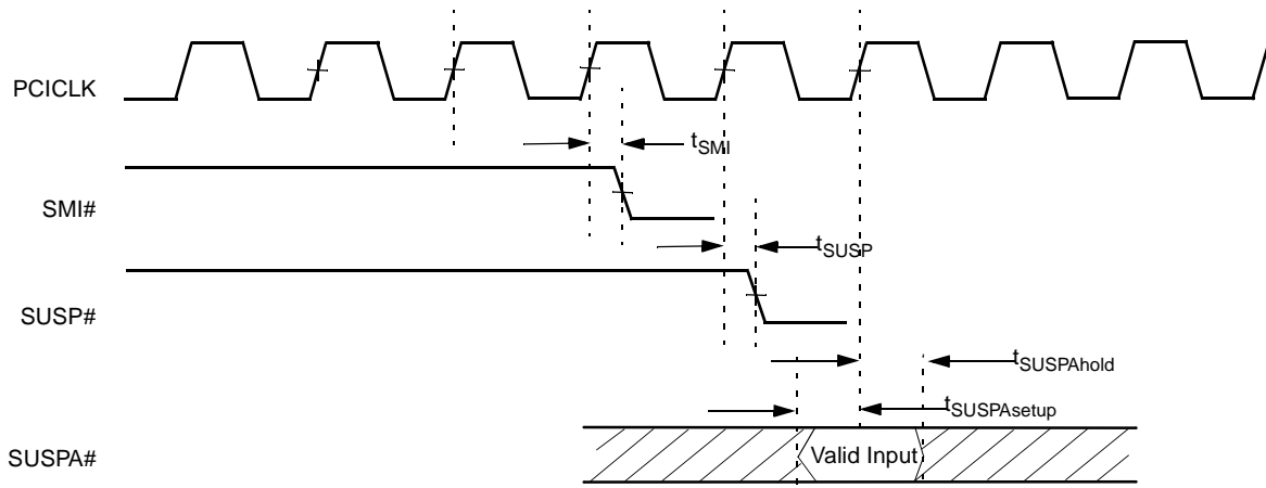
Figure 5-7. CPU Interface Timing
