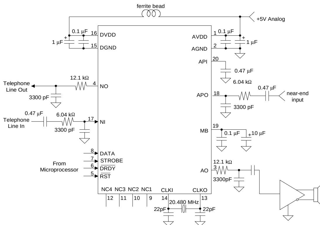
Figure 3. Typical Connection Diagram (Microphone Preamplifier Disabled)
