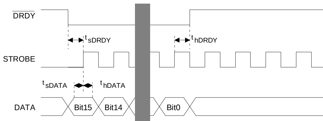
Figure 1. Microcontroller Interface Switching Characteristics
