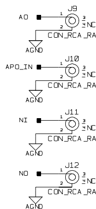
Figure 2. RCA Connections
