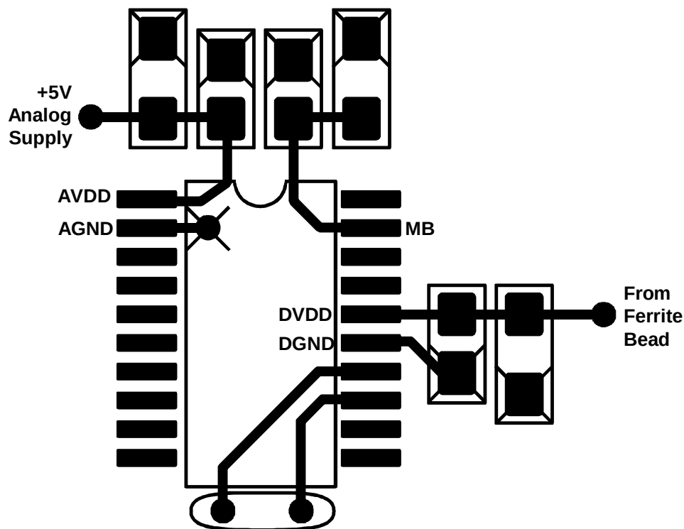
Figure 6. Suggested Layout
