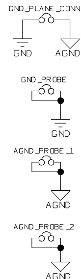
Figure 7. Grounds
