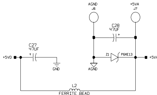
Figure 1. Power Supply
