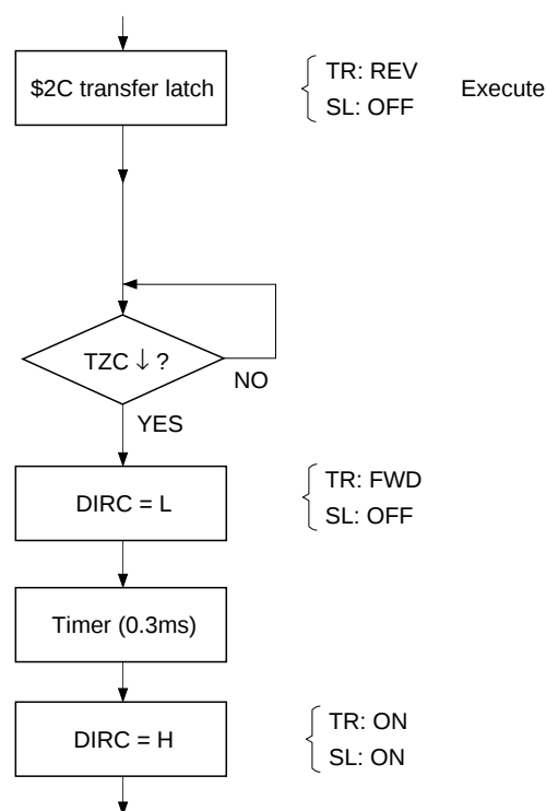
Fig. 10. 1-track jump with DIRC (Pin 20)
