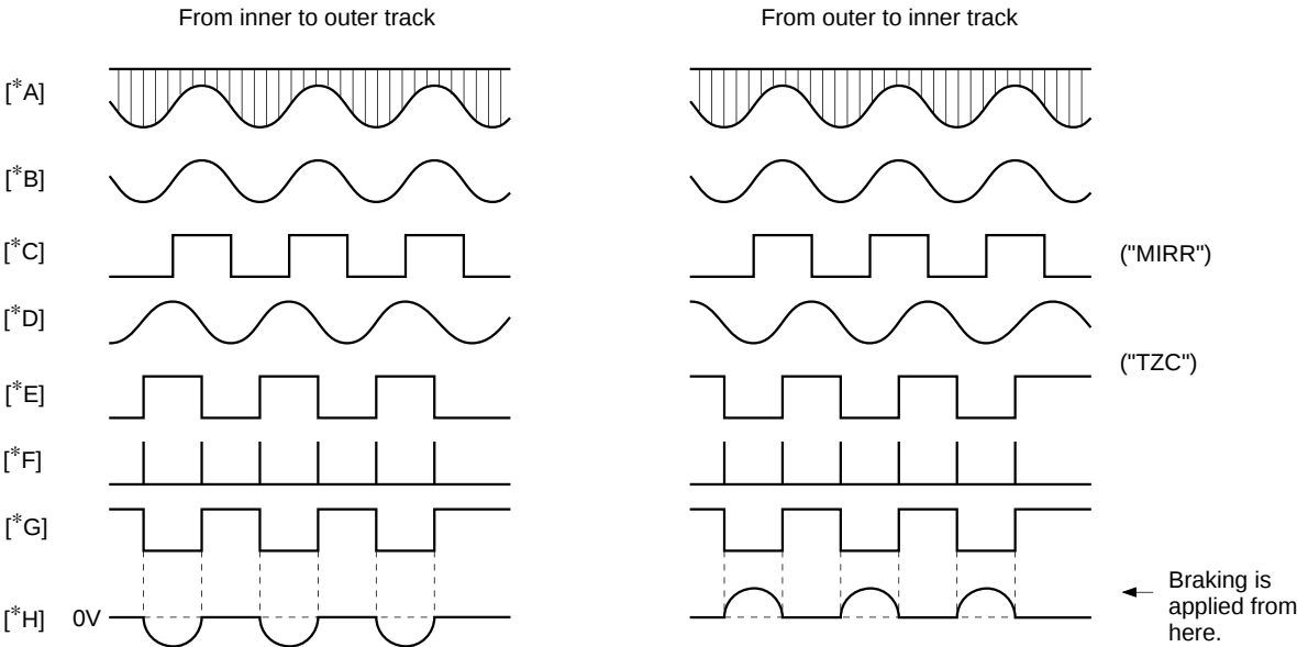
Fig. 7. Internal waveform
