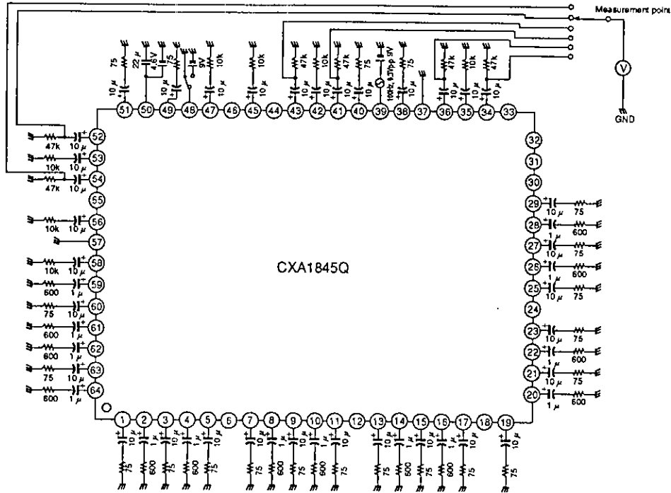
A f=100\text{Hz} , 0.3\text{Vp-p} signal is applied to Vcc and the output signals from Pins 34, 39, 41, 43, 52 and 54 are measured. When 9V is applied to Pin 48, the signals from Pins 32 and 34 can be measured for output gain of -6\text{dB} .
