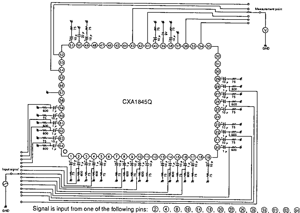
Fig. 4 Audio system (cross talk)
