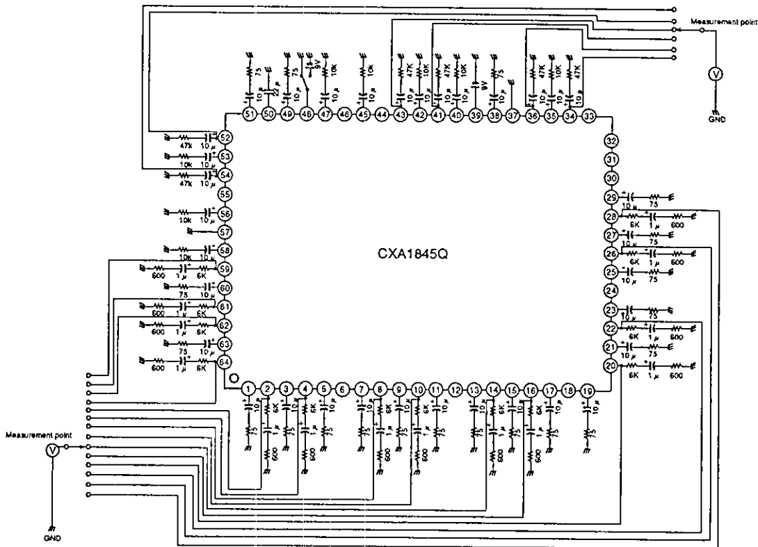
When 9V is applied to Pin 10, the signals from Pins 32 and 54 can be measured for output gain of -6\text{dB} .
