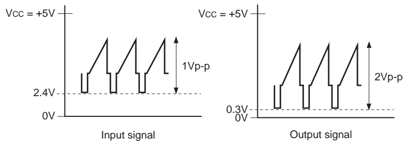
Fig. 10. CVBS/Y Waveforms
