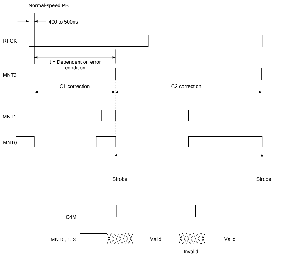
Timing Chart 3-3
