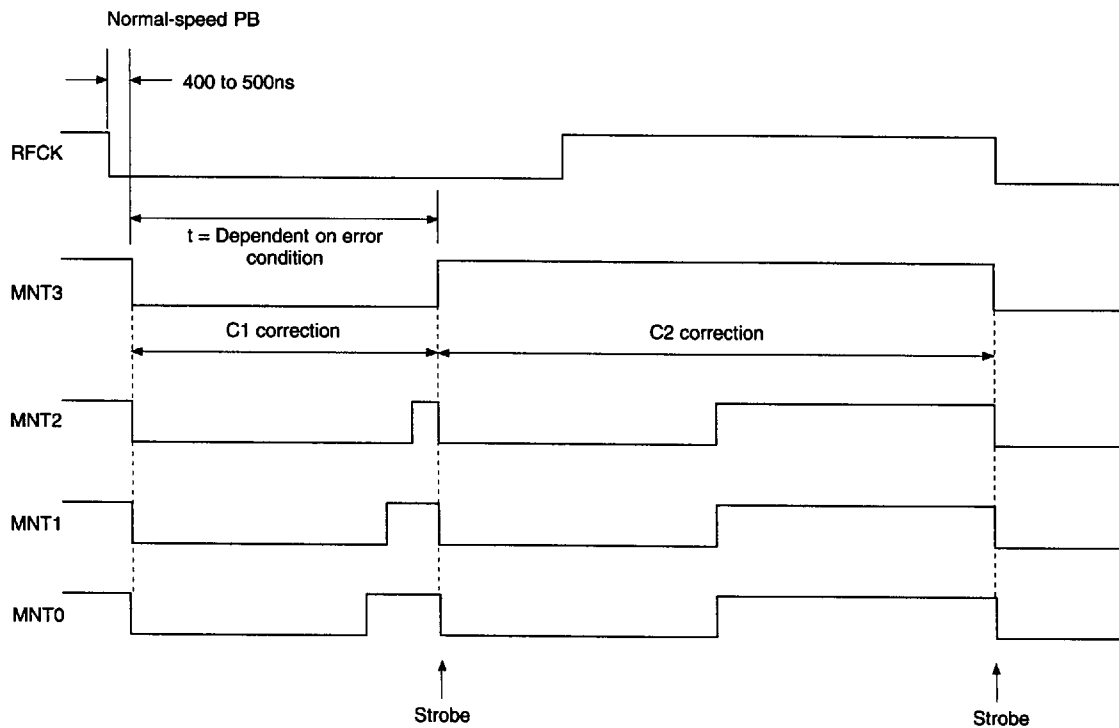
Timing Chart 3-3
