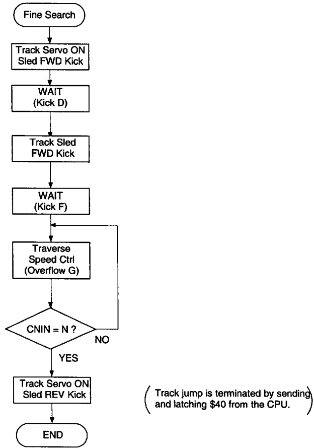
Fig. 3-12. (a) Fine Search Flow Chart
