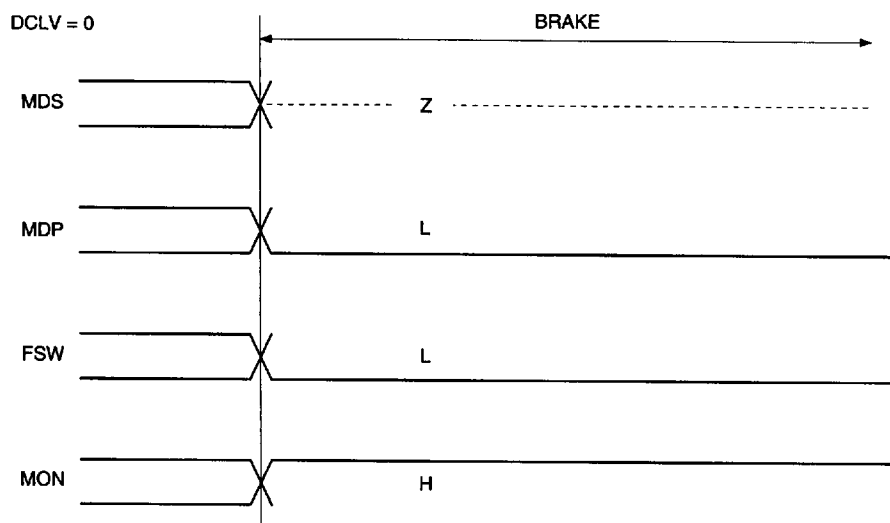
Timing Chart 1-9
