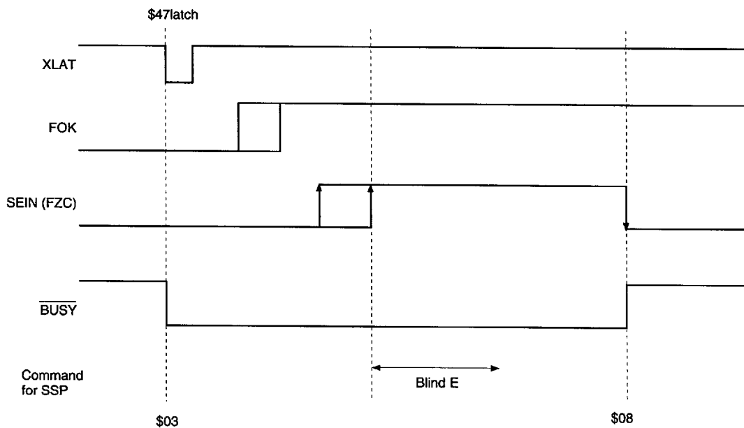
Fig. 3-8. (b) Auto Focus Timing Chart
