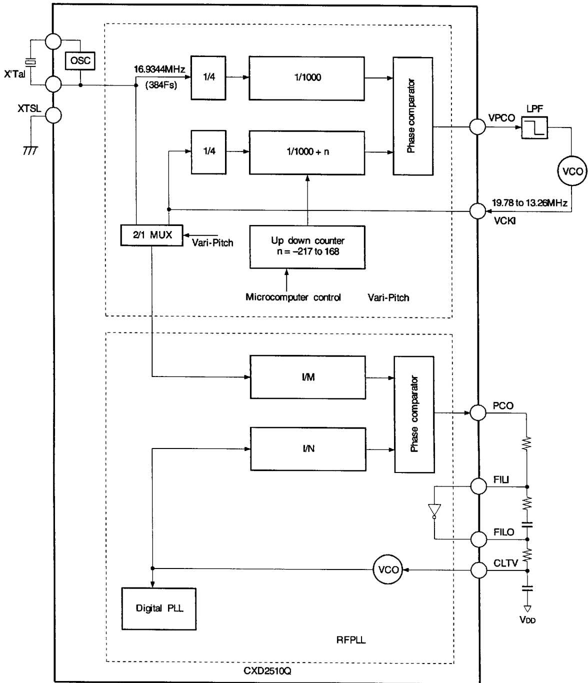
Block Diagram 3-1
