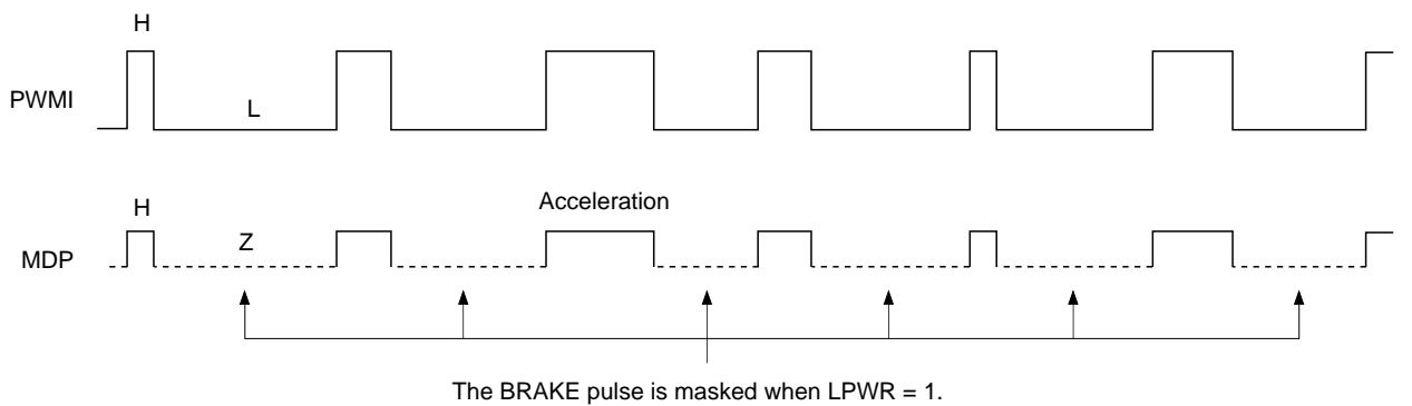
Timing Chart 1-15
