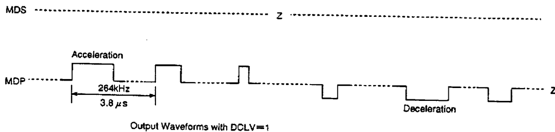
Timing Chart 1-16
