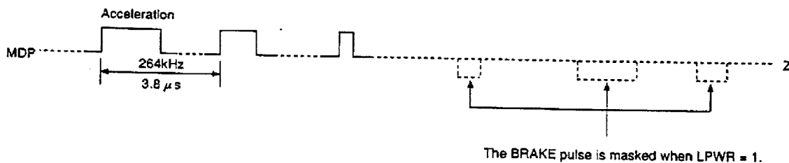
Timing Chart 1-18
