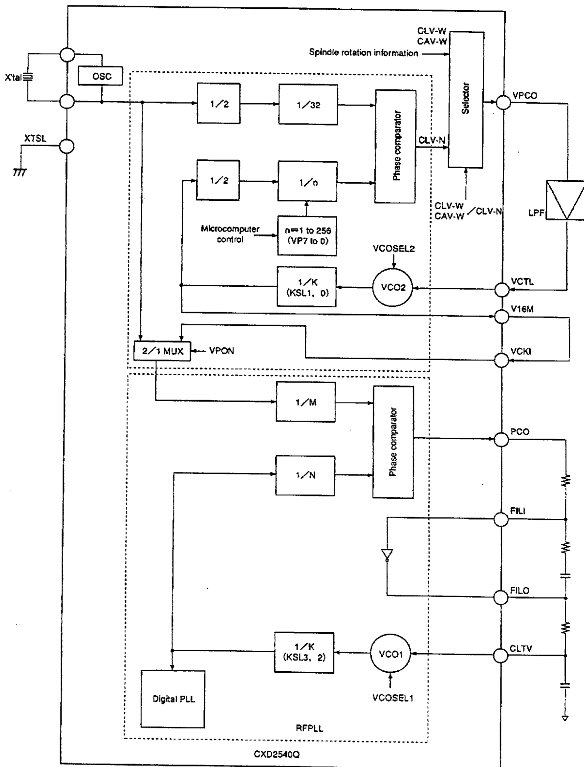
Block Diagram 3-1
