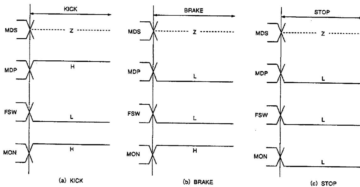
Timing Chart 1-7
