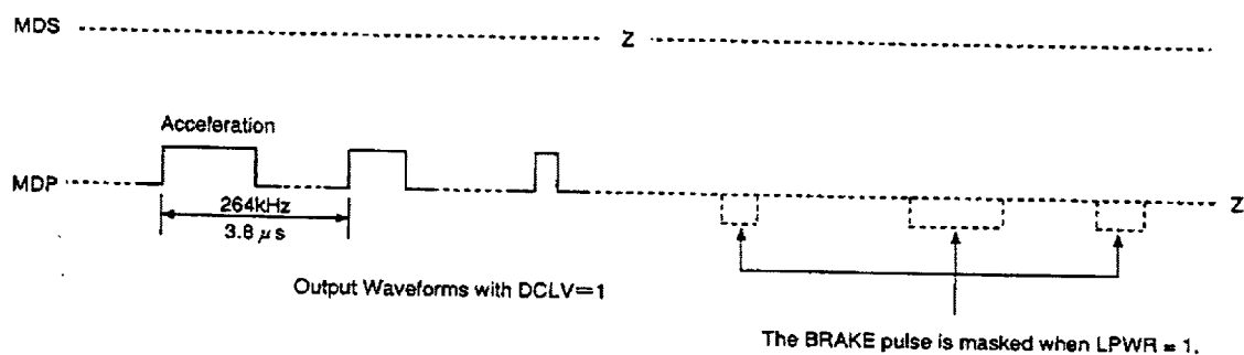
Timing Chart 1-17
