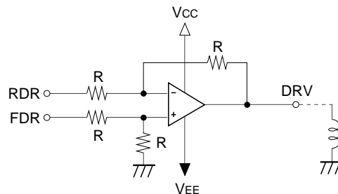
Fig. 5-21. Drive Circuit
