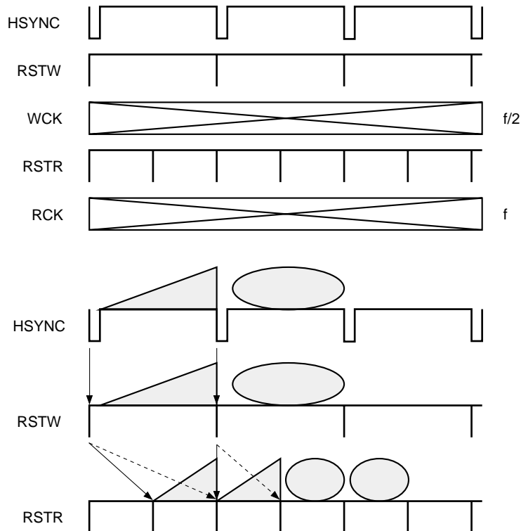
Double-speed display timing
