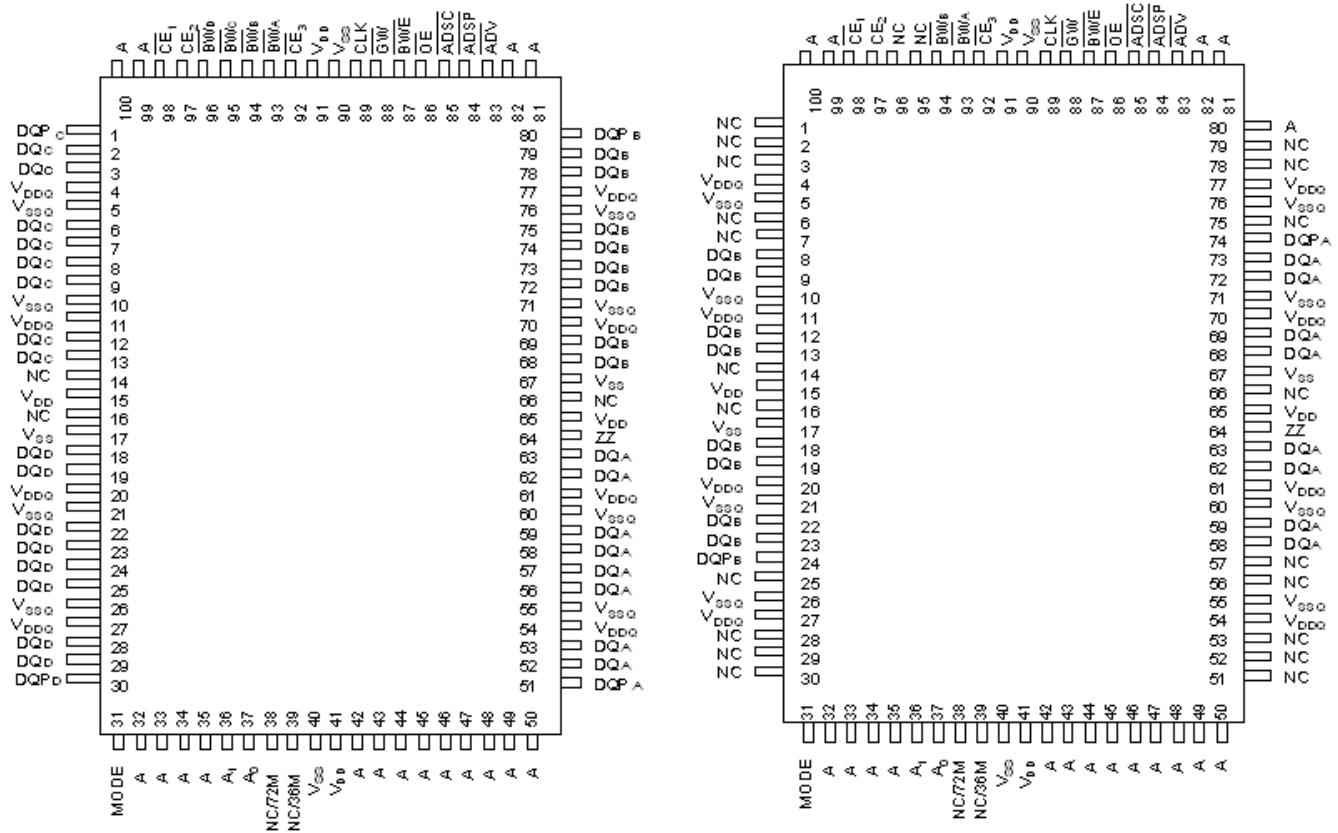
CY7C1380D (512 K × 36)
