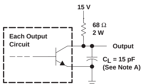
TEST CIRCUIT
