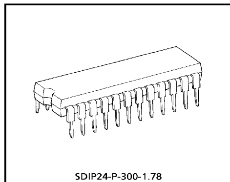
SDIP24-P-300-1.78
