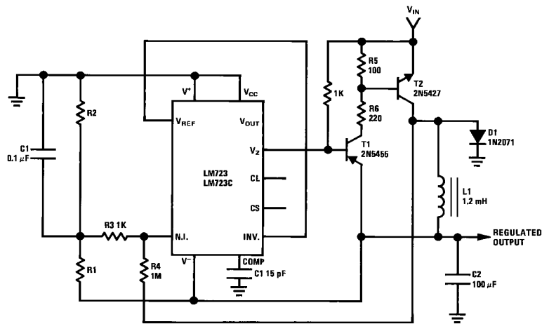
FIGURE 9. Positive Switching Regulator
