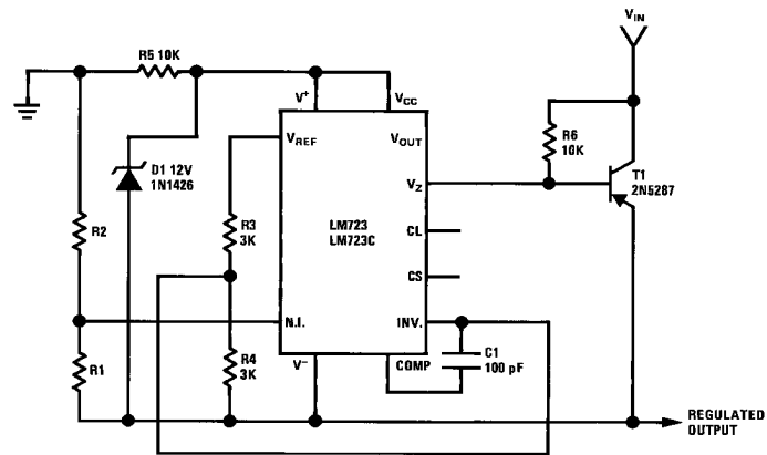
FIGURE 7. Positive Floating Regulator
