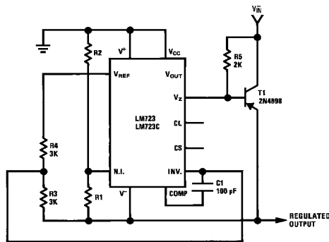
FIGURE 2. Basic High Voltage Regulator ( V_{OUT} = 7 to 37 Volts)
