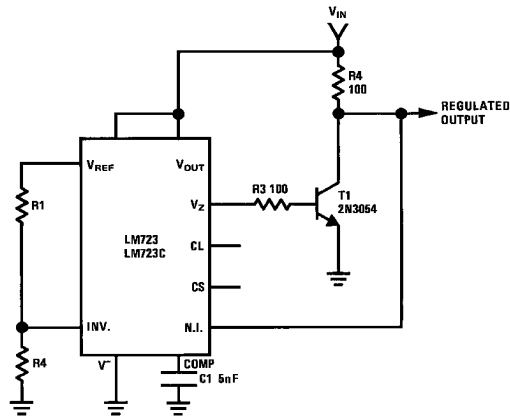
FIGURE 11. Remote Shutdown Regulator with Current Limiting
