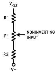
FIGURE 13. Output Voltage Adjust (Note 6)
