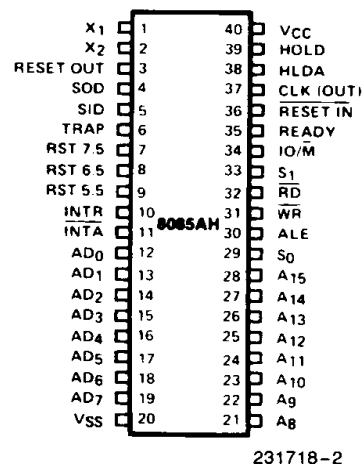
Figure 2. 8085AH Pin Configuration
