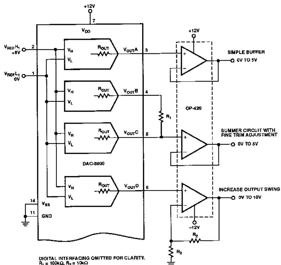
FIGURE 7: Buffering the DAC-8800 Output
