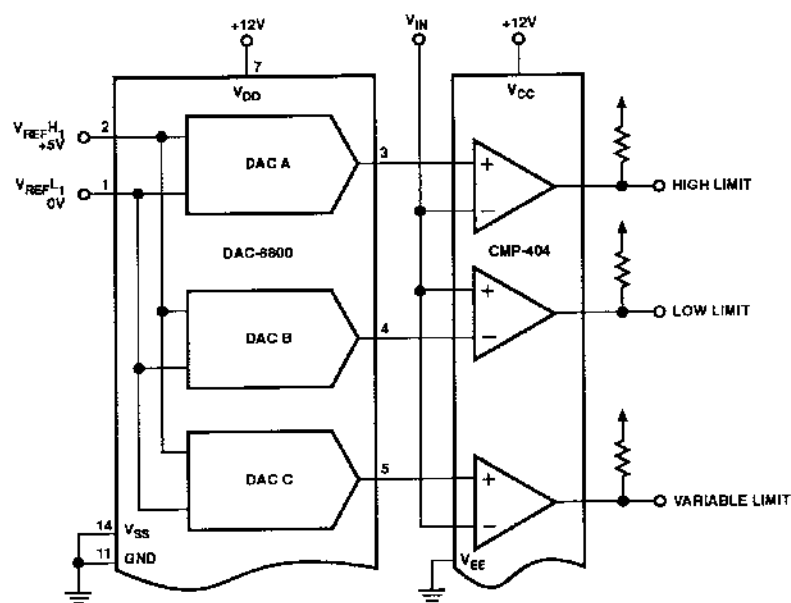
FIGURE 8: Setting the Comparator Trip Points
