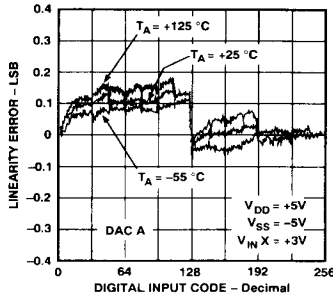
Figure 3. Linearity Error vs. Digital Code vs. Temperature
