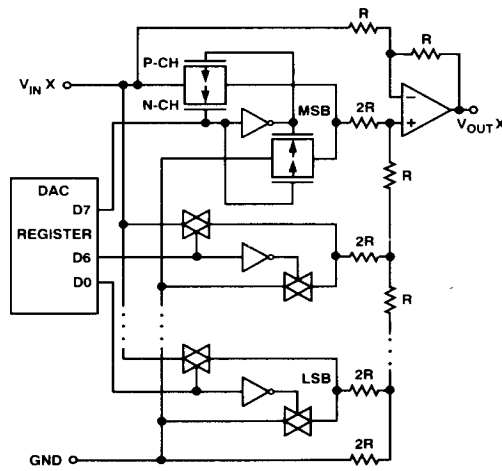
Figure 24. DAC-8840 TrimDAC Equivalent Circuit
