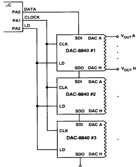
Figure 26. Three-Wire Interface Updates Multiple DAC-8840s
