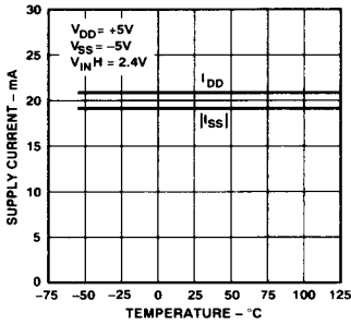
Figure 18. Supply Current vs. Temperature
