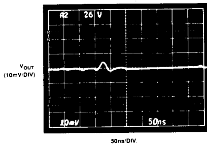
Figure 15. Digital Crosstalk
