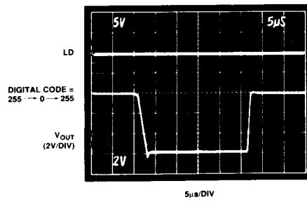
Figure 12. Settling Time
