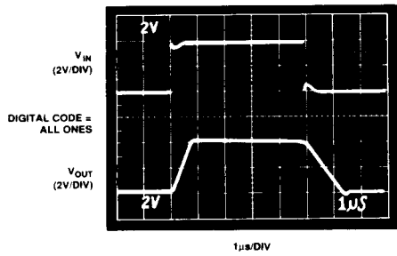
Figure 11. Pulse Response
