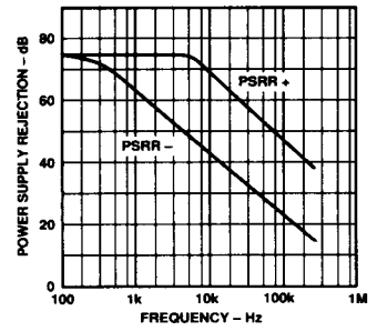
Figure 20. PSRR vs. Frequency
