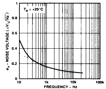
Figure 10. Voltage Noise Density vs. Frequency
