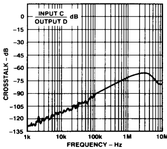
Figure 9. DAC Crosstalk vs. Frequency
