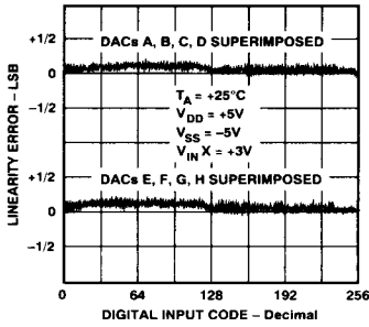
Figure 2. Linearity Error vs. Digital Input Code
