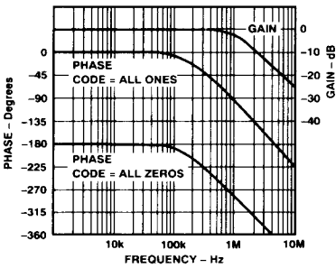
Figure 8. Gain and Phase vs. Frequency (Digital Input = 0 or 255_{10} )
