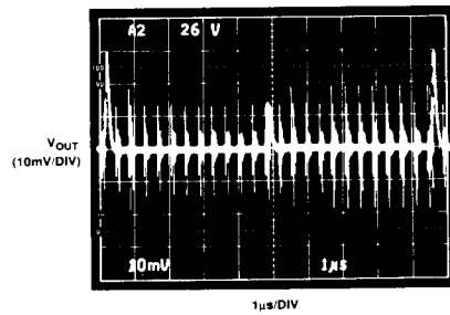
Figure 16. Clock Feedthrough
