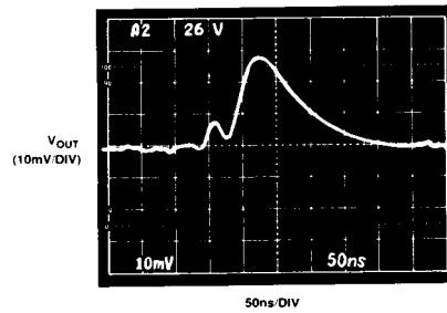
Figure 14. Digital Feedthrough
