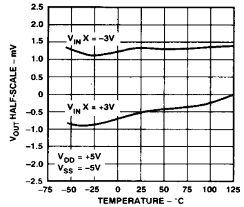
Figure 4. V_{OUT} Half-Scale ( 80_H ) vs. Temperature
