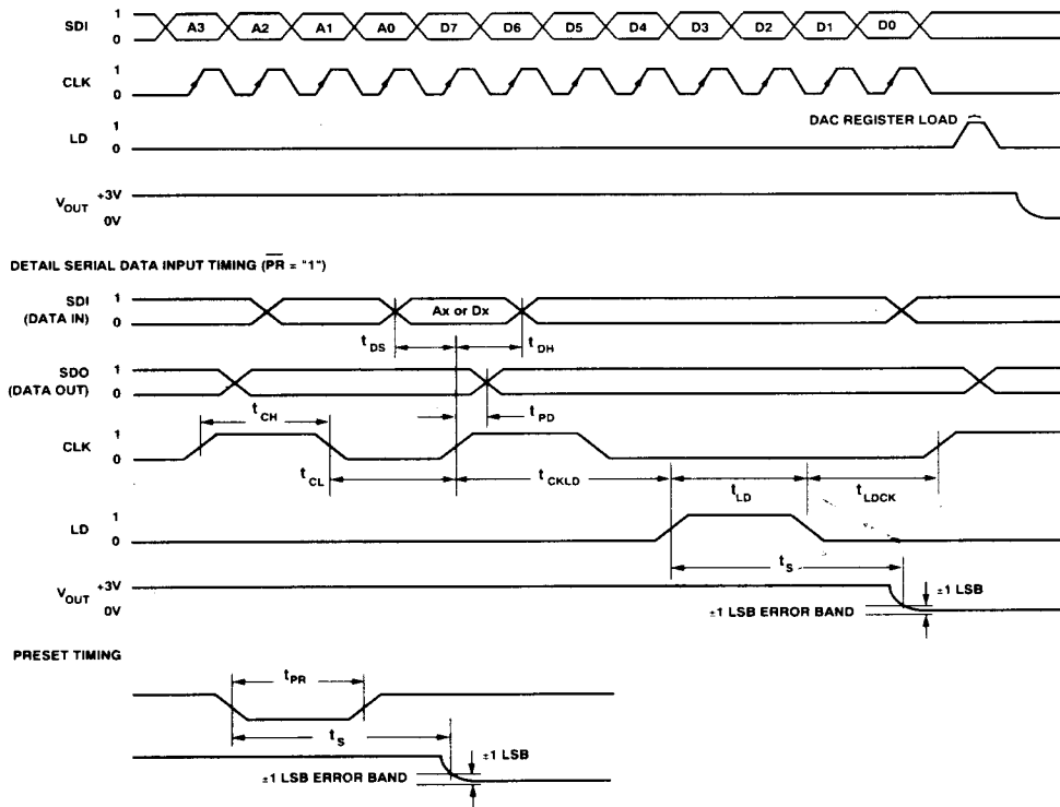
Figure 1. Timing Diagram
