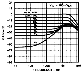
Figure 21. Gain ( V_{OUT}/V_{IN} ) and Feedthrough vs. Frequency
