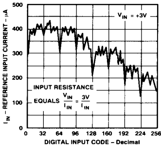
Figure 5. Input Resistance vs. Code
