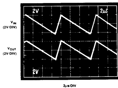
Figure 17. 128 kHz Sawtooth Waveform
