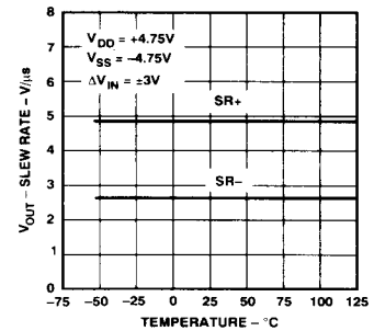
Figure 7. V_{OUT} Slew Rate vs. Temperature
