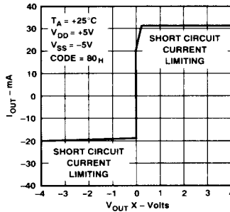
Figure 22. DAC Output Current vs. V_{OUT}X
