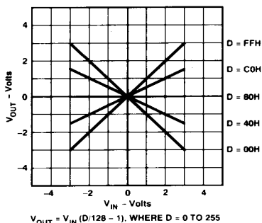
Figure 25. DAC Plus Amplifier Combine to Produce Four Quadrant Multiplication
