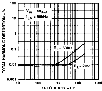
Figure 6. Total Harmonic Distortion vs. Frequency
