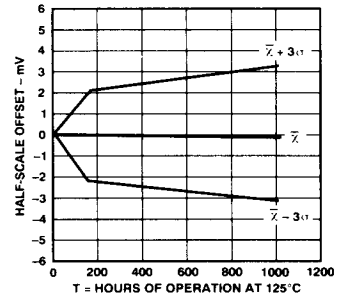
Figure 23. Output Drift Delta Accelerated by Burn-In
