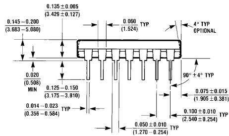
14-Lead Molded Dual-In-Line Package (N) Order Number DM74LS14N Package Number N14A
