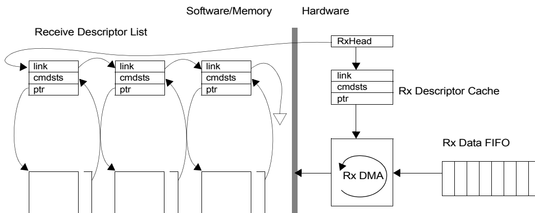
Figure 5-6 Receive Architecture
