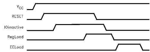
FIGURE 6. RESET Operation
