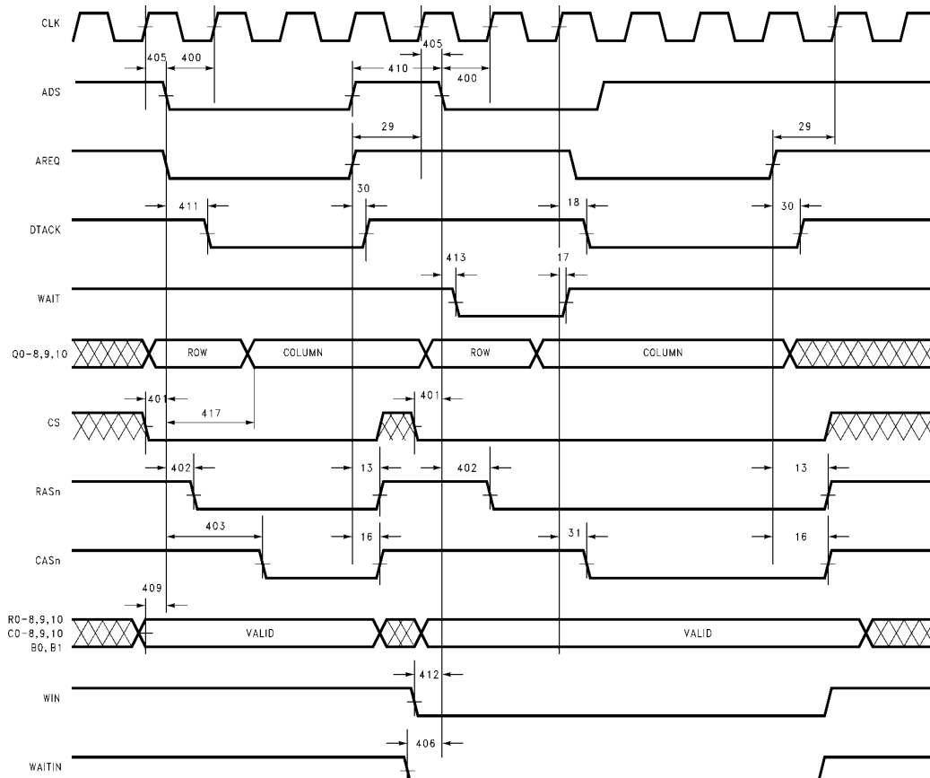
FIGURE 42. 400: Mode 1 Timing
