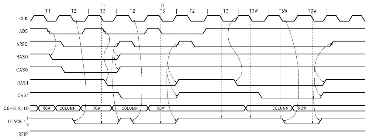
FIGURE 11d. Mode 1 Address Pipelining (DTACK 1/2T Programmed, DTACK is Sampled at the "T3" Falling Clock Edge)
