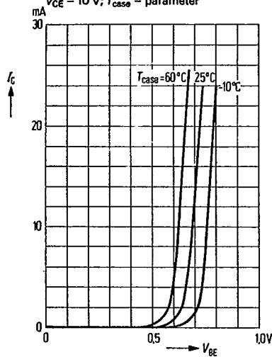
Collector current I_C = f(V_{BE}) V_{CE} = 10\text{ V}; T_{case} = \text{parameter}
