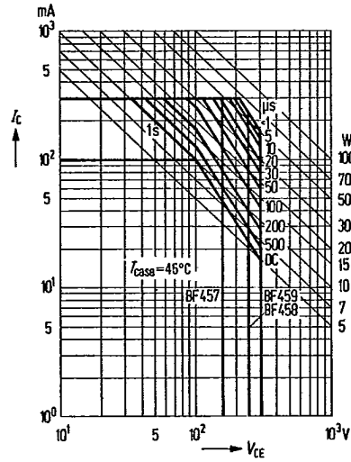
Permissible operating range I_C = f(V_{CE}) ; T_{case} = 45^{\circ}C ; v = 0.1
