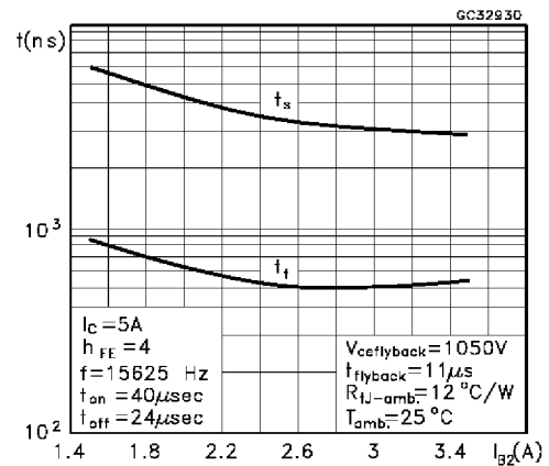
Switching Time Inductive Load at 16KHz (see figure 2)
