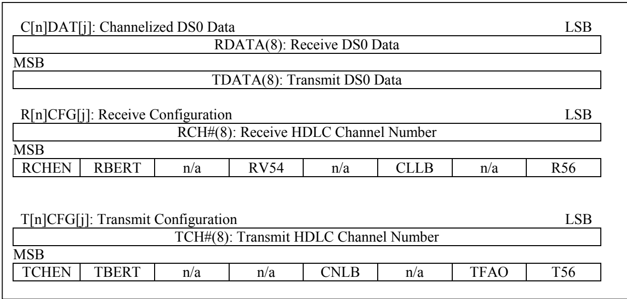
Figure 6-3. Layer 1 Register Set
