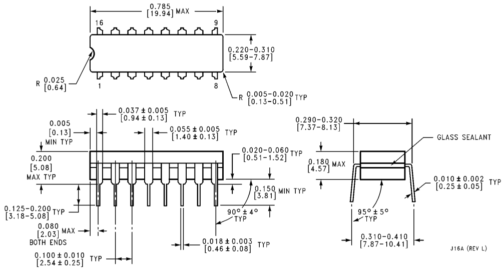
Ceramic Dual-In-Line Package (J) Order Number DS3662J NS Package Number J16A
