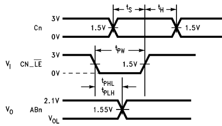
TL/F/10721-4 FIGURE 2. Driver: CN_LLE to AB7, t_s , t_H , t_{pw}
