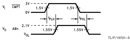
TL/F/10721-5 FIGURE 3. Driver: CMPT to AB7
