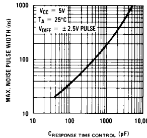
Noise Rejection
