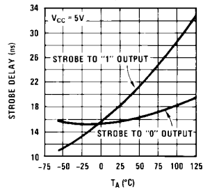
Strobe Delays
