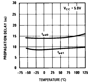
Propagation Delay from Input to Output (Channel 2)
