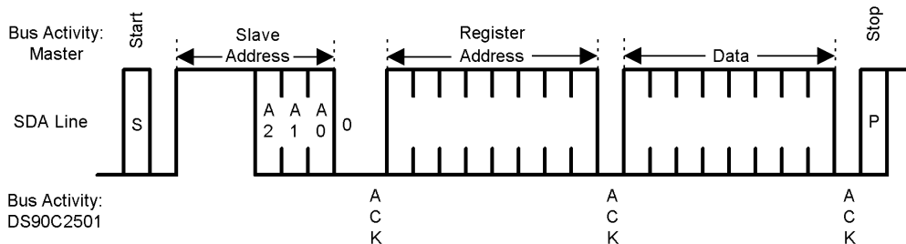
FIGURE 13. Byte Write
