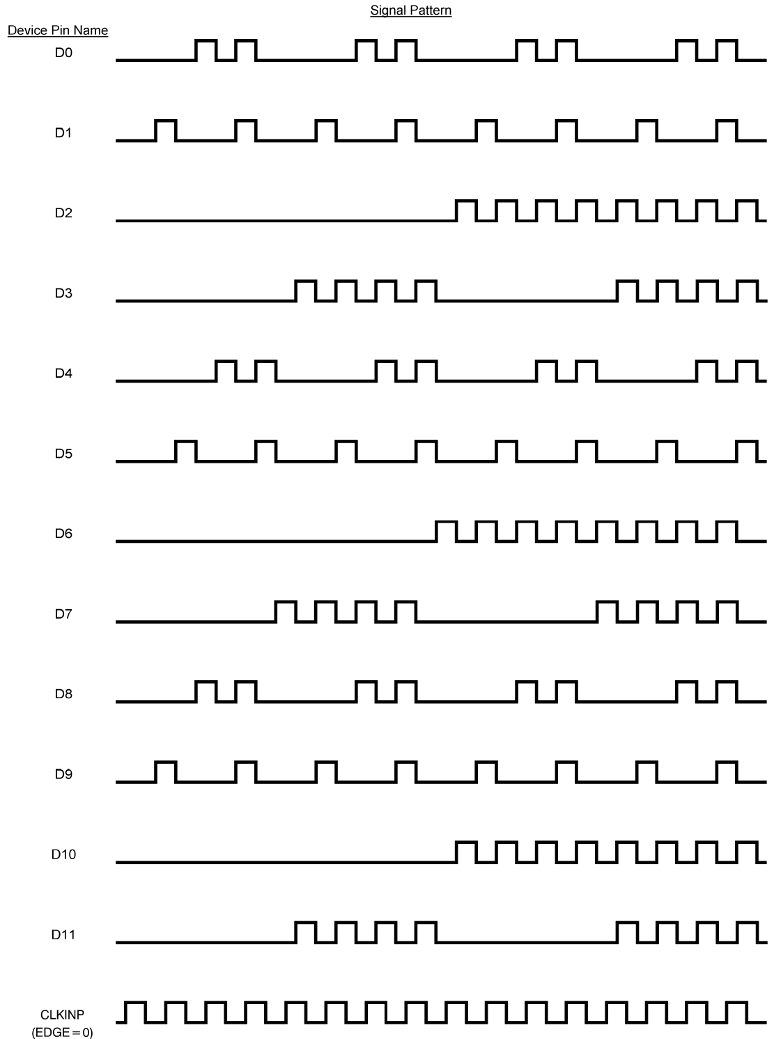
FIGURE 2. "16 Grayscale" Test Pattern in 12-bit Input Mode(Note 9)
