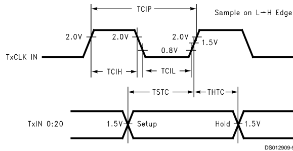
FIGURE 6. D590CR215 (Transmitter) Setup/Hold and High/Low Times
