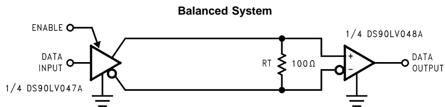
FIGURE 5. Point-to-Point Application
