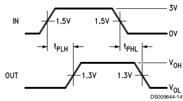
FIGURE 8. Receiver Propagation Delay Times
