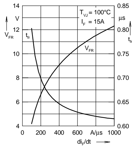
Fig. 6 Peak forward voltage V_{FR} and t_{rr}
